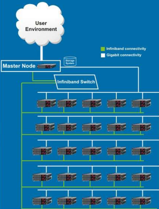
HCL-HPC block architecture
